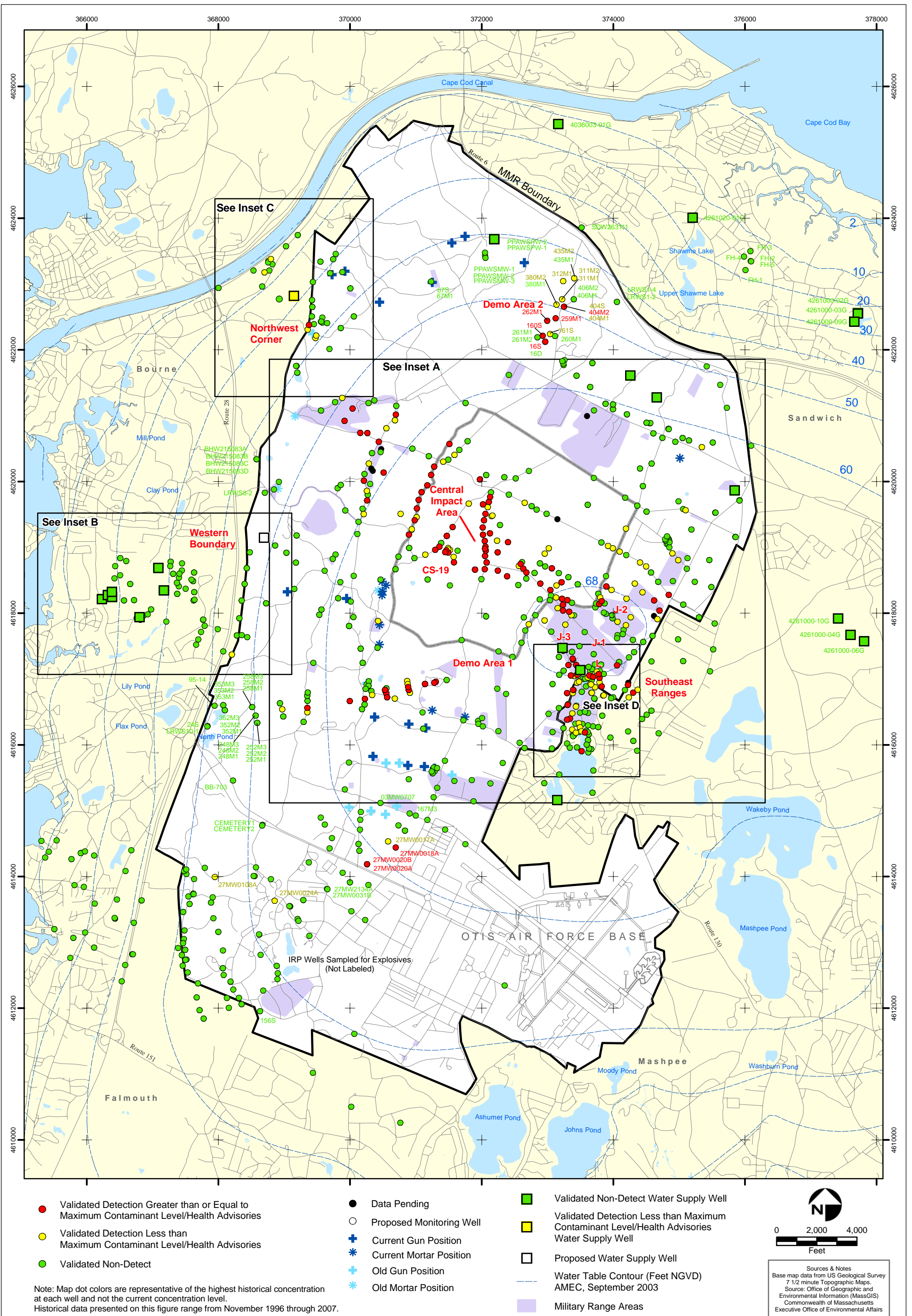
Explosives in Groundwater Compared to Maximum Contaminant Level/Health Advisories Validated Data as of 5/25/07
